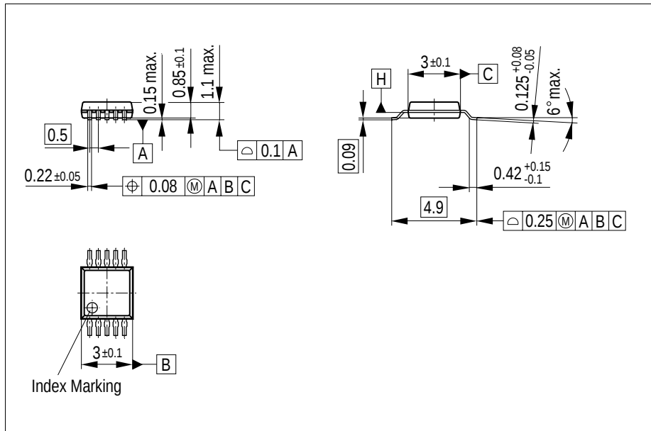
Figure 15 PG-TSSOP-10
