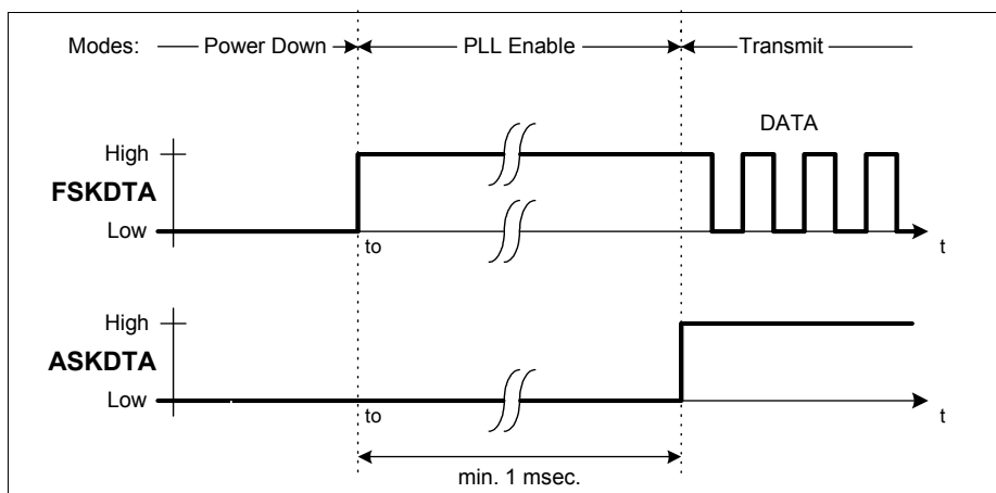
Figure 5 FSK Modulation
