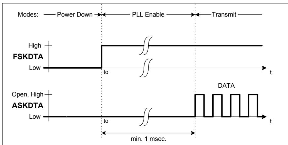
Figure 4 ASK Modulation
